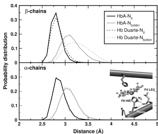
FIGURE 12 Probability distribution of the distances N_{\delta} (His F8)-CO(Leu F4) (black curves) and N_{bckbn} (His F8)-CO(Leu F4) (gray curves) for the deoxy Hbs. The solid and dotted curves refer to data for HbA and Hb Duarte, respectively. In the inset, the N ions and the leucine residue involved in the formation of H-bonds are shown.
