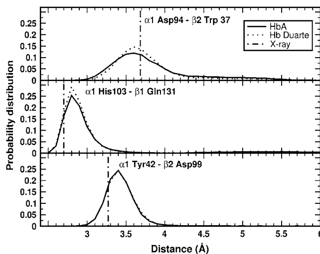
FIGURE 11 Probability distributions of the distances in the switch region of the deoxy Hbs: (upper panel) Asp-94–Trp-37 at the \alpha_1\beta_2 interface; (central panel) His-103–Gln-131 at the \alpha_1\beta_1 interface; (lower panel) Tyr-42–Asp-99 at the \alpha_1\beta_2 interface. Solid and dotted curves are for HbA and Duarte variants, respectively. The dash-dot lines indicate the corresponding distances in the x-ray structures.
