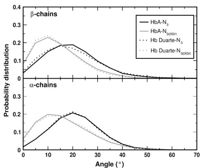
FIGURE 13 Probability distribution of the angles N_{\delta} (His F8)-CO(Leu F4) (black curves) and N_{bckbn} (His F8)-CO(Leu F4) (gray curves) for the deoxy Hbs. The solid and dotted curves refer to data for HbA and Hb Duarte, respectively.
